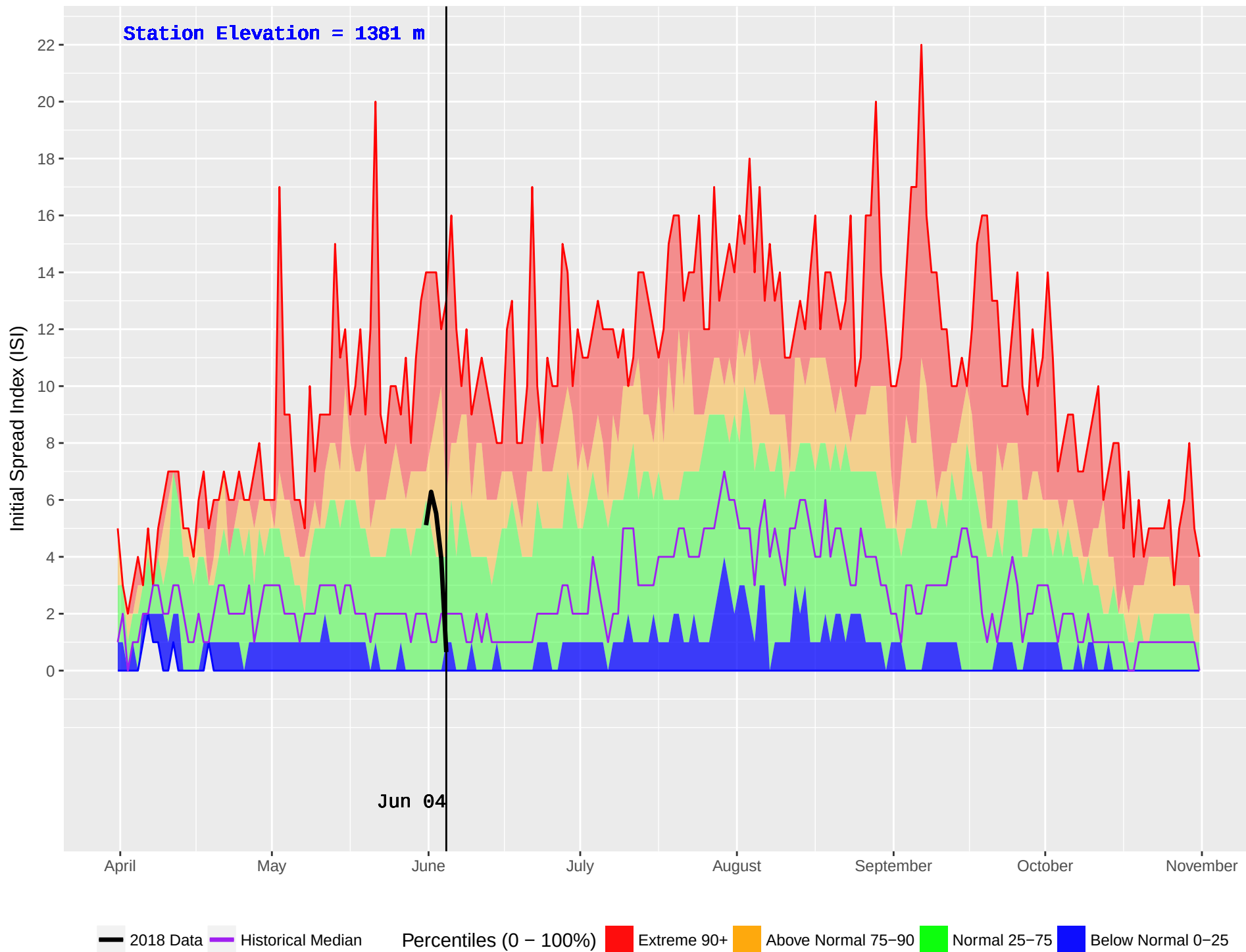
GLIMPSE (291) : Historical (1978–2016) and Current (2018) Noon Initial Spread Index (ISI)
